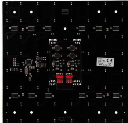
LED-Tile C25 MK2.6 (rear view)
